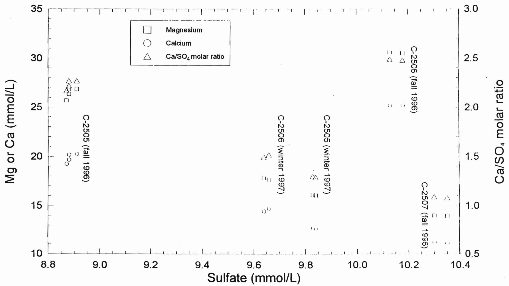
Figure 4.3. Variation of Ca/SO 4 molar ratio and magnesium and calcium concentrations with sulfate concentration.
