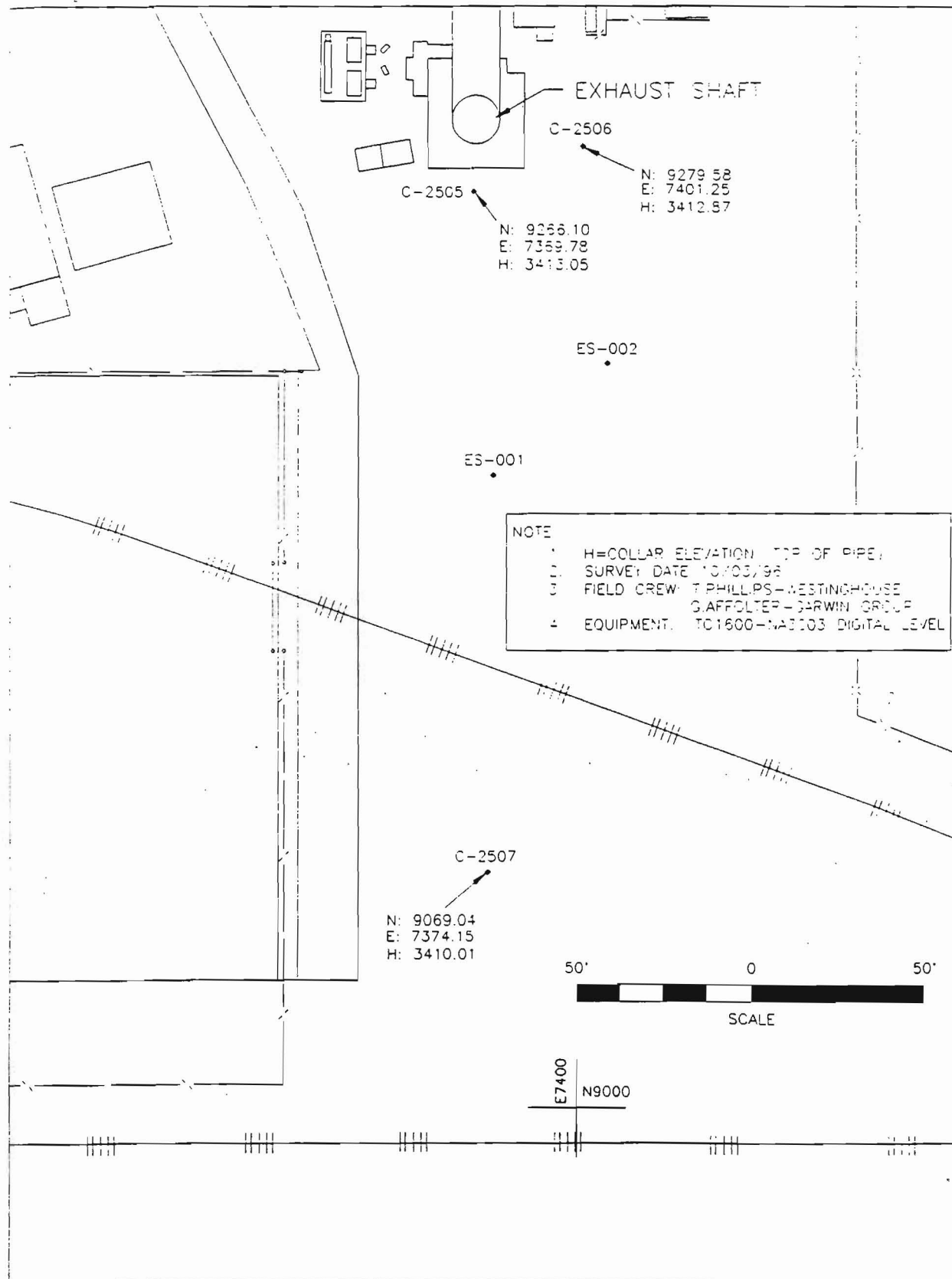
Figure 1.1. Location of boreholes C-2505, C-2506, and C-2507.
