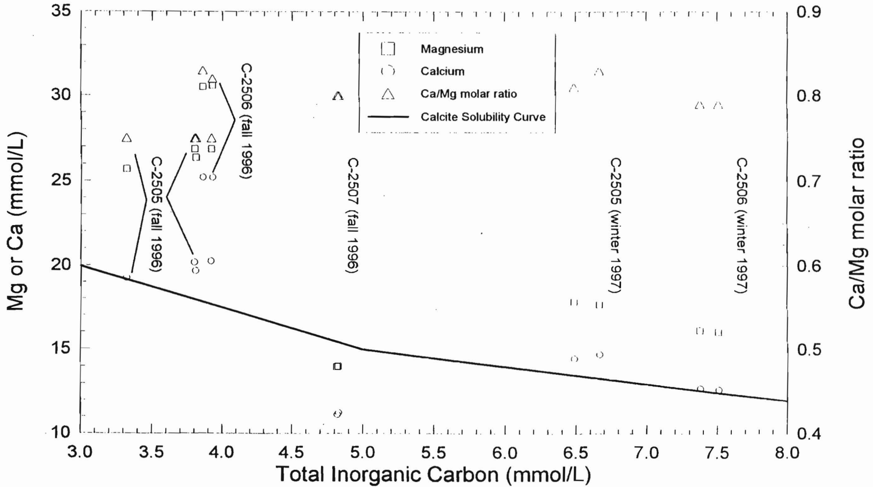
Figure 4.4. Variation of Ca/Mg molar ratio and magnesium and calcium concentrations with total inorganic carbon (TIC).
