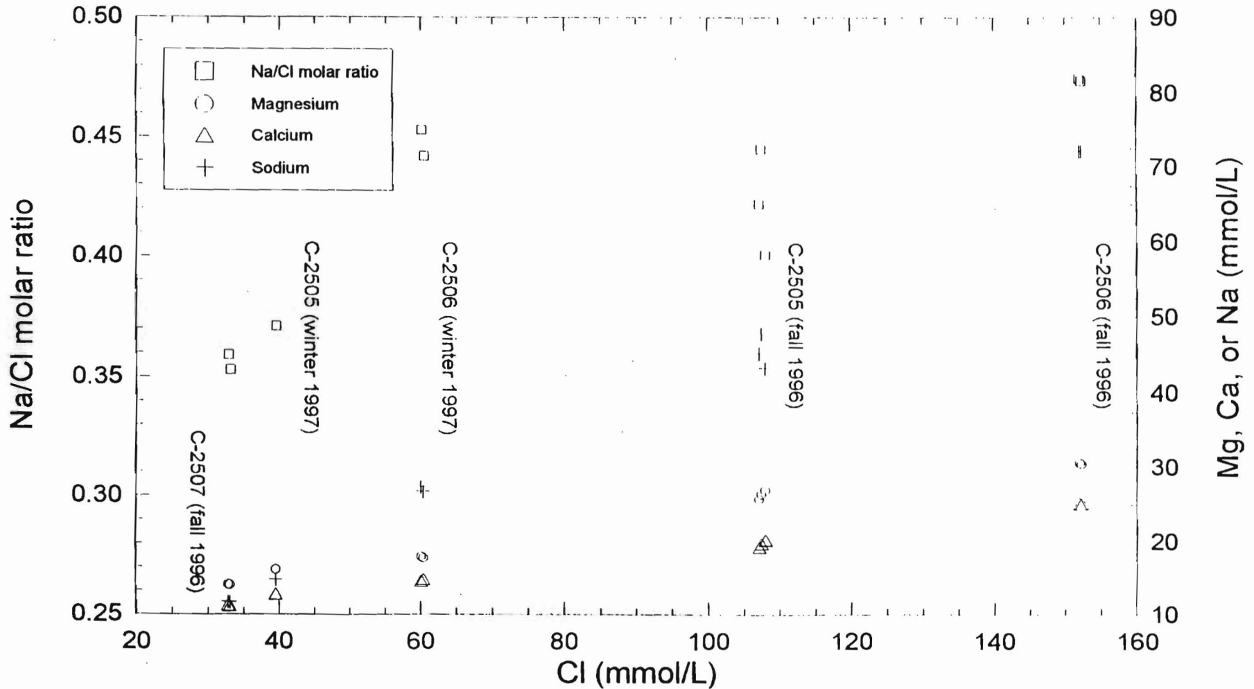
Figure 4.2. Variation of Na/Cl molar ratio and magnesium, calcium, and sodium concentrations with chloride concentration.
