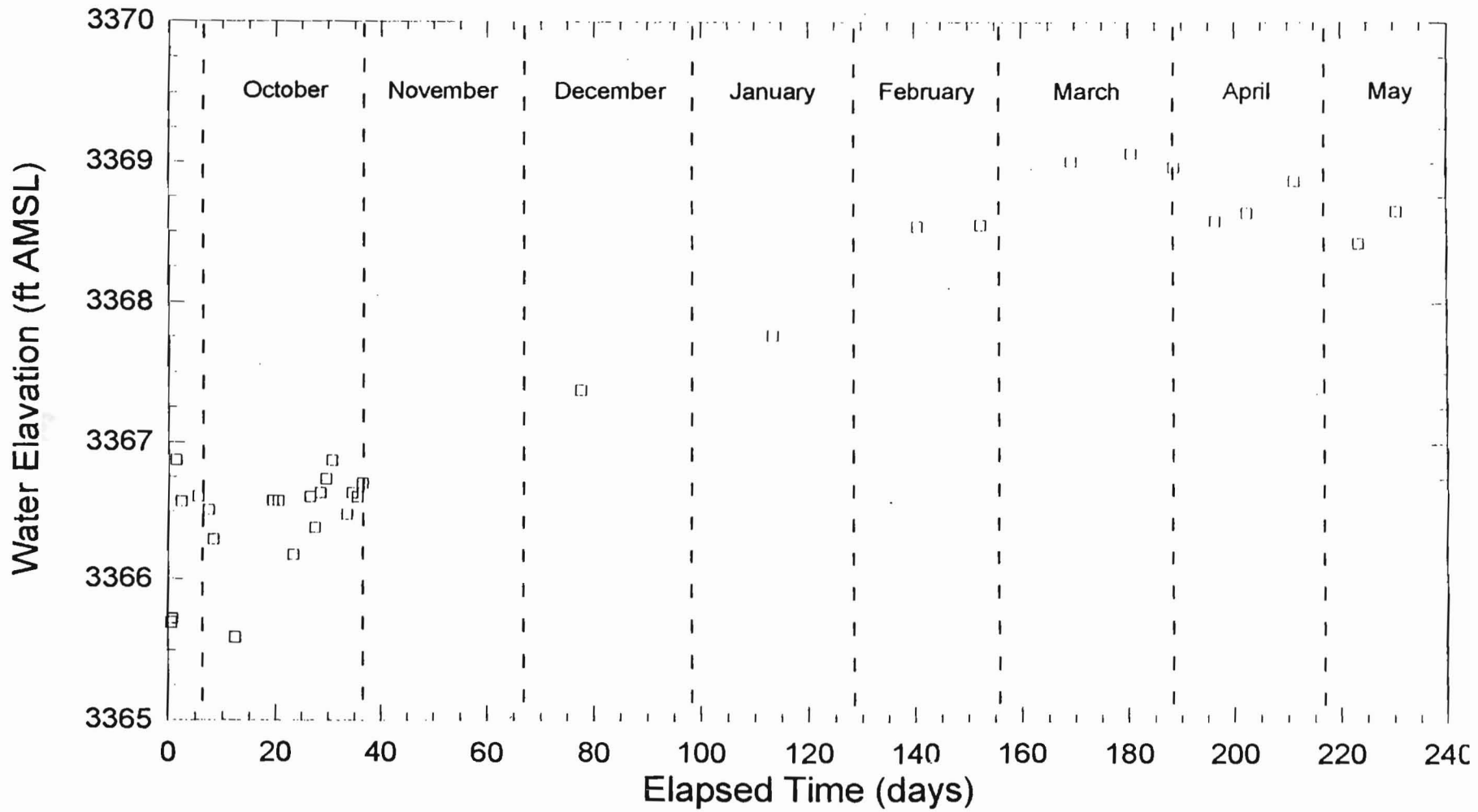
Figure 3.16. C-2506: water level versus time.
