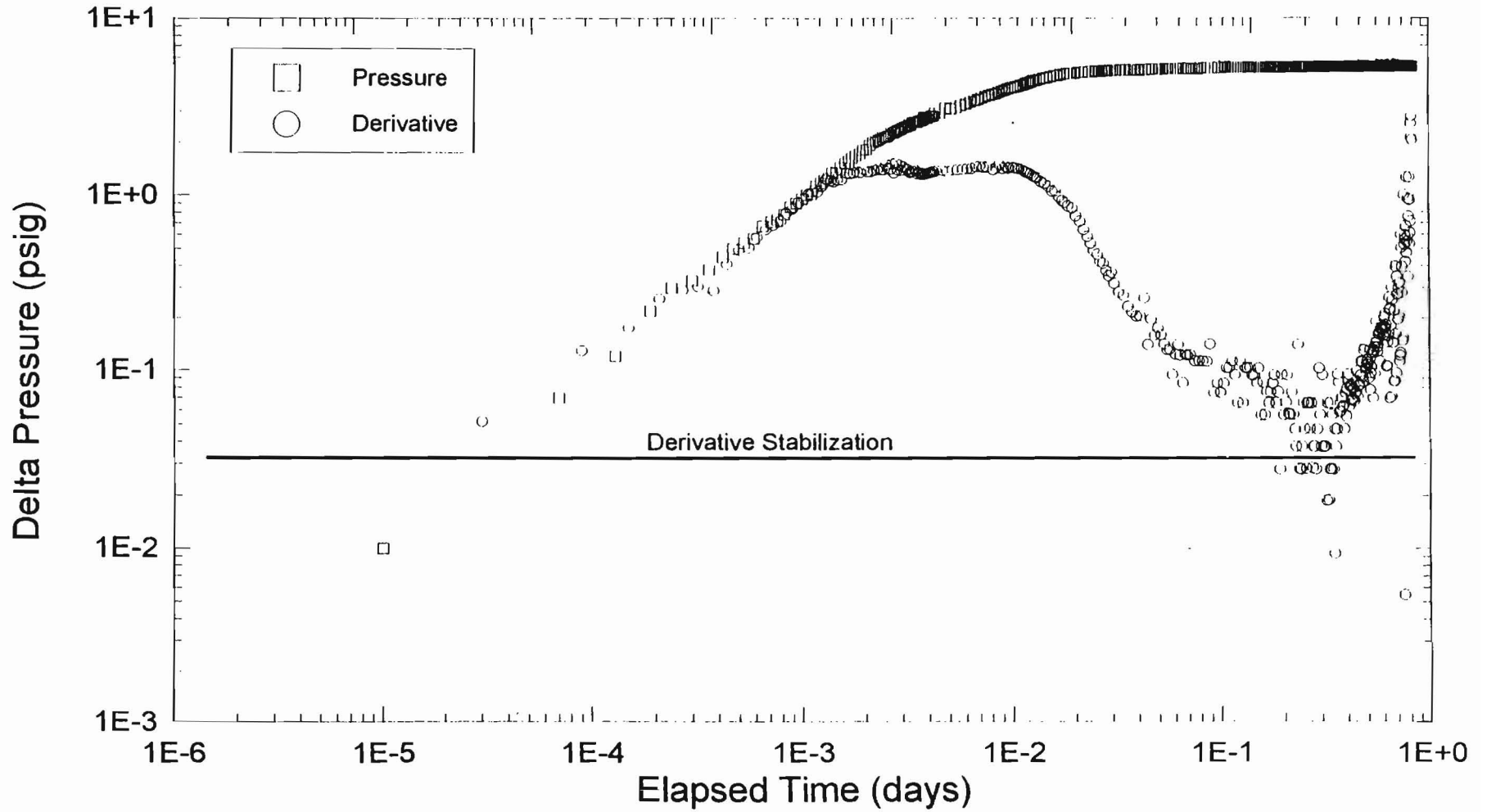
Figure 3.3. C-2506 pumping test #2: diagnostic derivative plot (recovery period).
