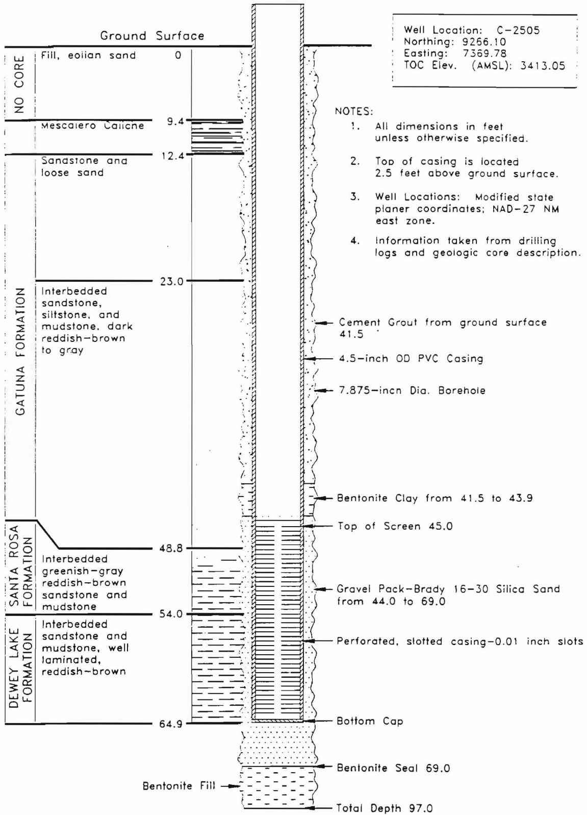
Figure 2.1. C-2505 well completion diagram.
