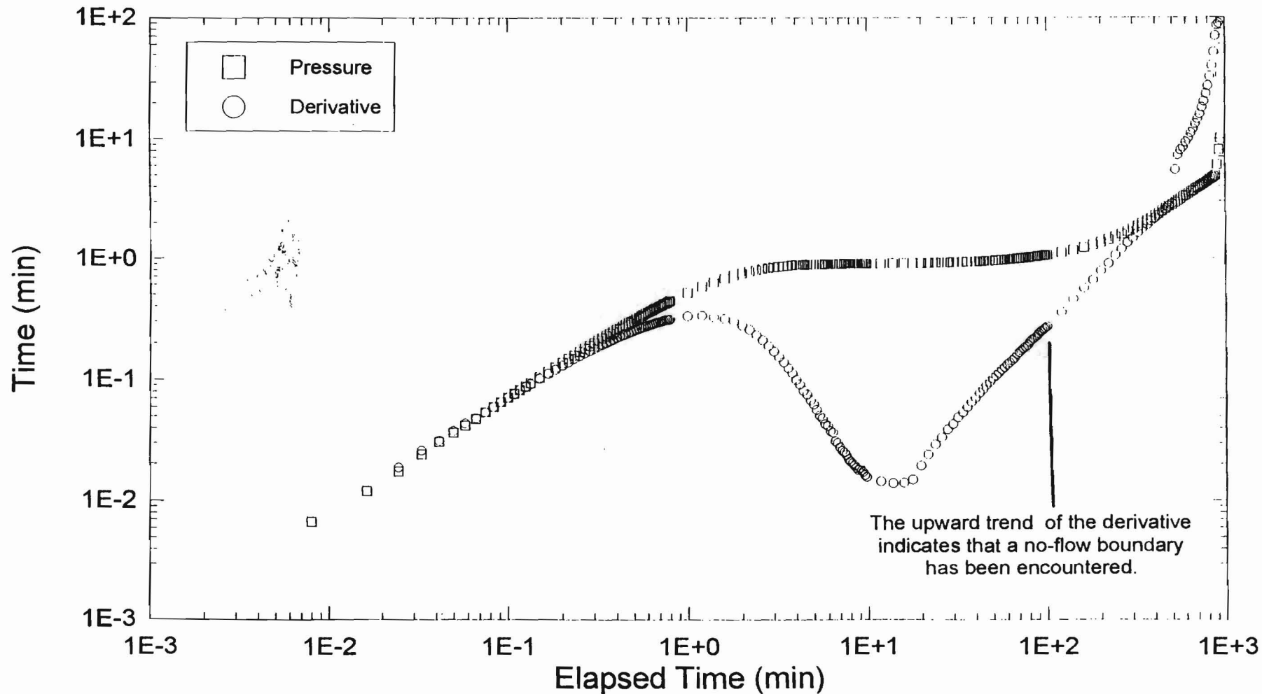
Figure 3.6. C-2506 slug test #2: equivalent diagnostic derivative plot.
