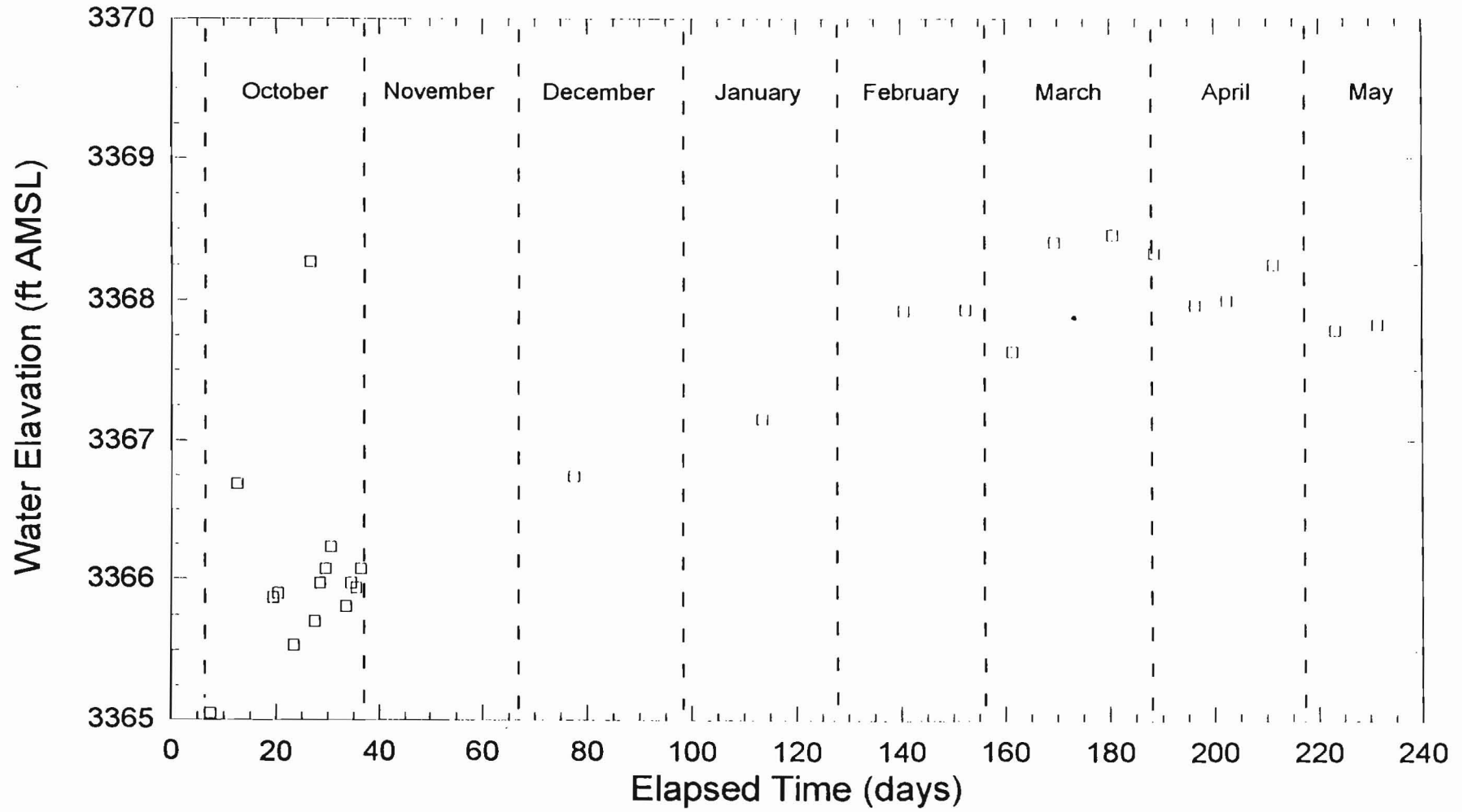
Figure 3.15. C-2505: water level versus time.
