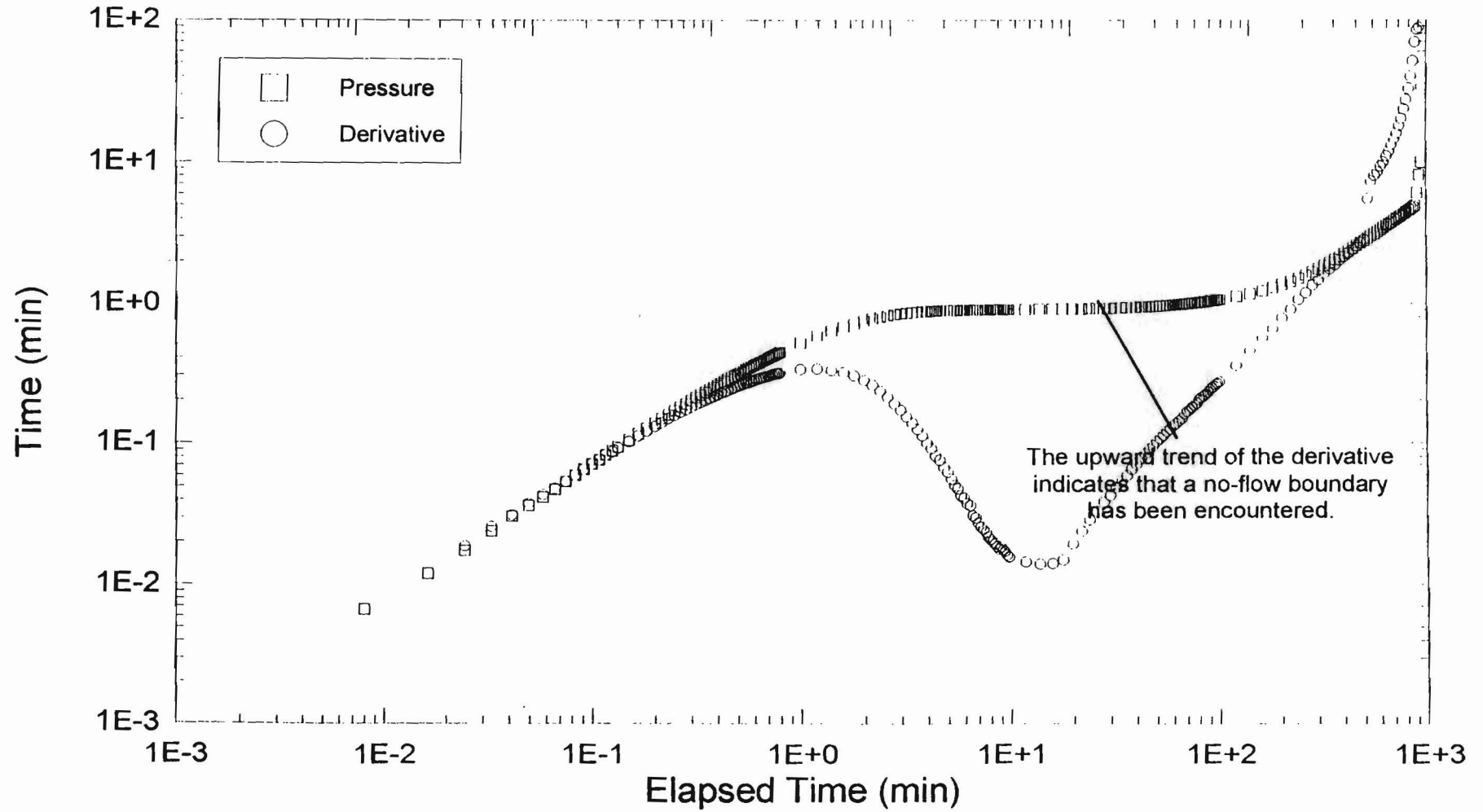
Figure 3.7. C-2507 slug test #2: equivalent diagnostic derivative plot.
