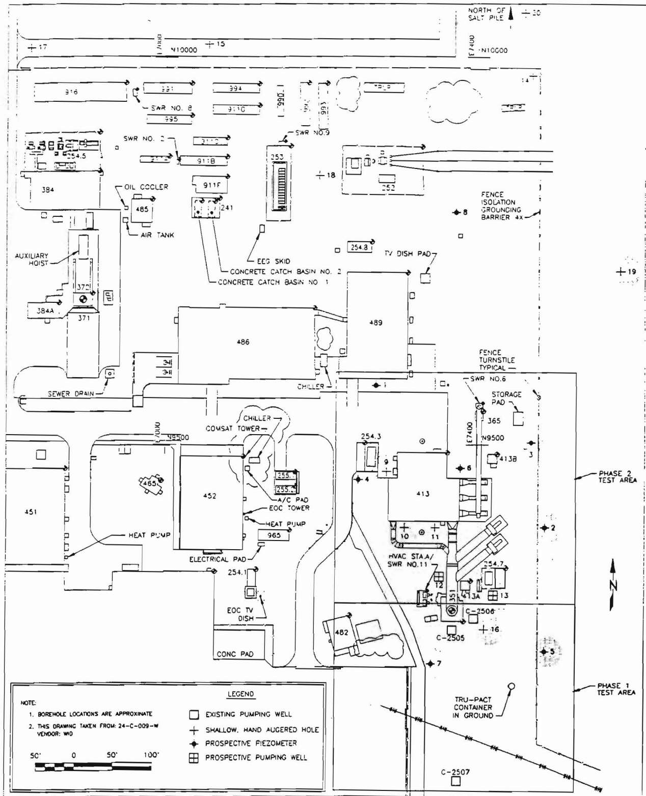
Figure 6.1. WIPP site map indicating shallow, hand augured boreholes, piezometers, and pumping wells associated with the Exhaust Shaft Assessment Program.
