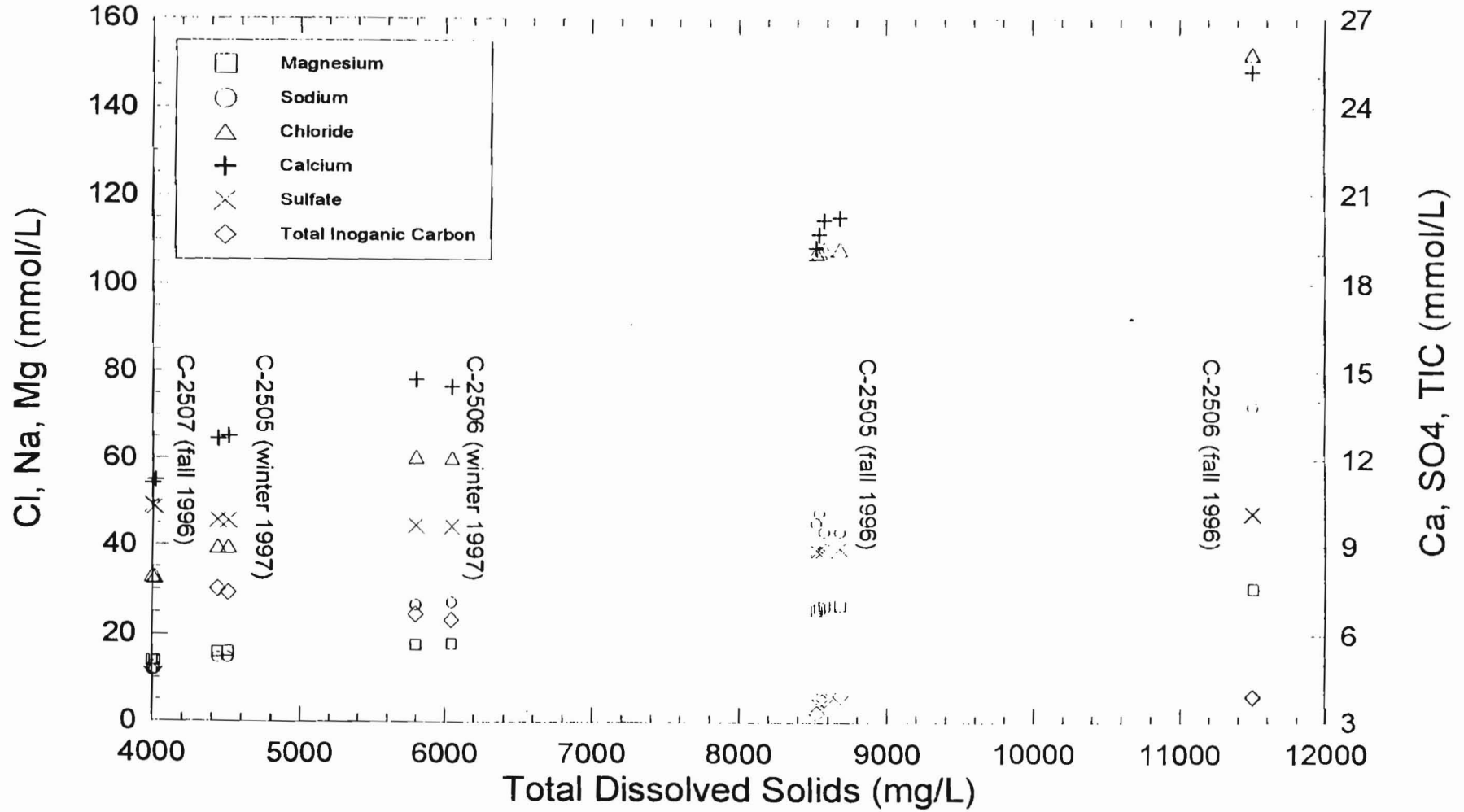
Figure 4.1. Major-ion concentrations versus total dissolved solids.
