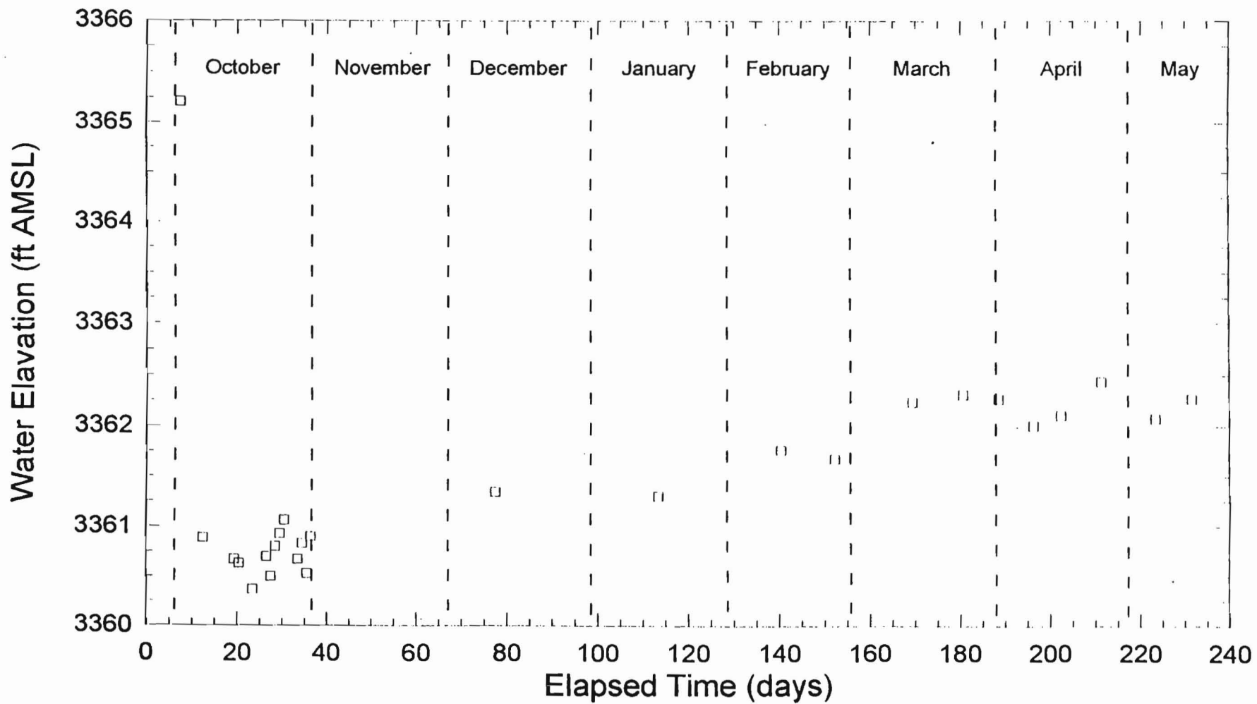
Figure 3.17. C-2507: water level versus time.
