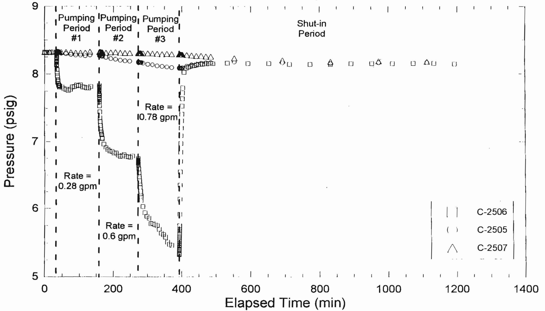
Figure 3.8. C-2506 pumping test #1: pressure versus time (C-2505, C-2506, and C-2507).
