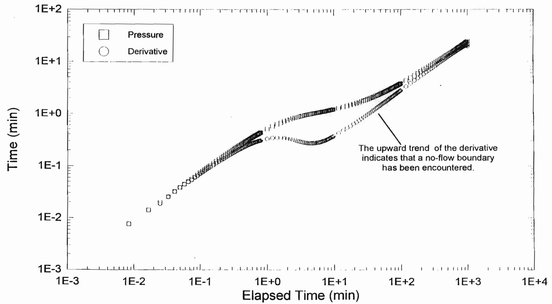
Figure 3.5. C-2505 slug test #1: equivalent diagnostic derivative plot.
