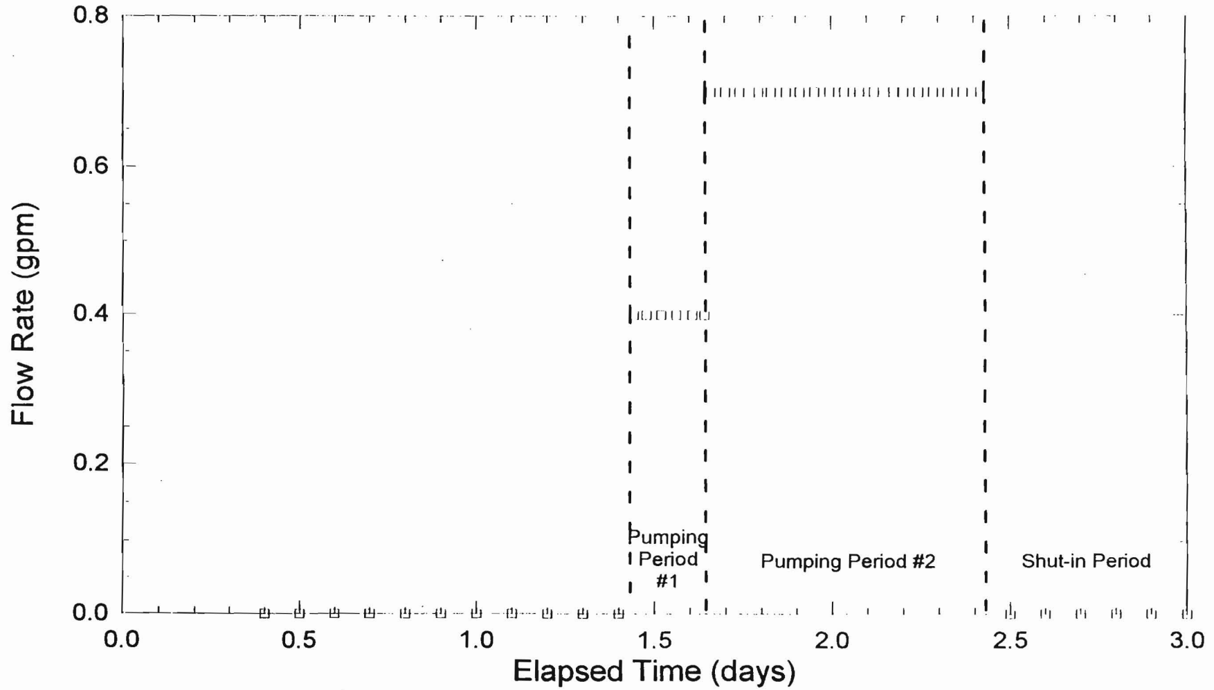
Figure 3.10. C-2505 pumping test: flow rate versus time.
