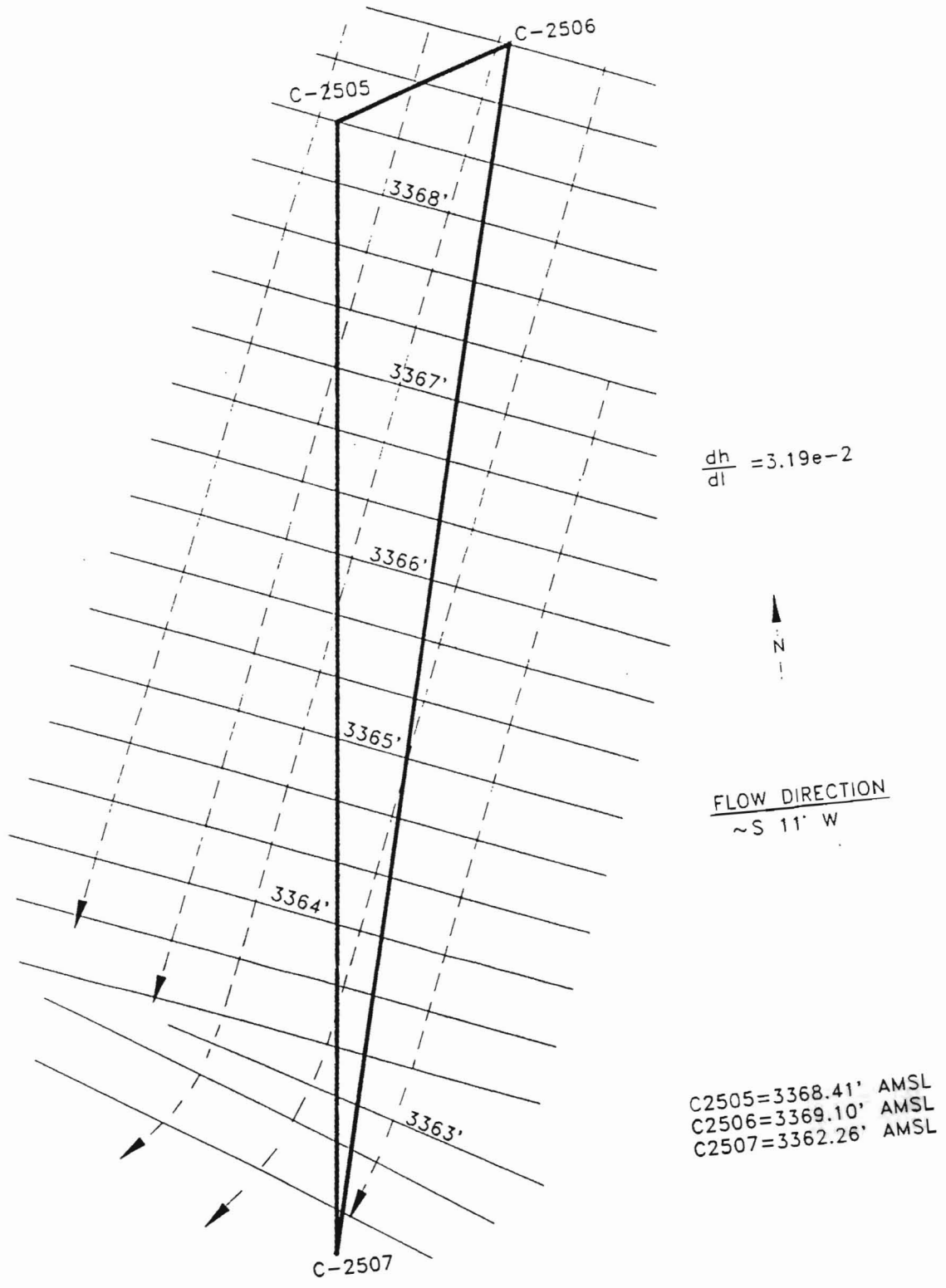
Figure 3.20. Equipotential and flow lines (March 13, 1997).
